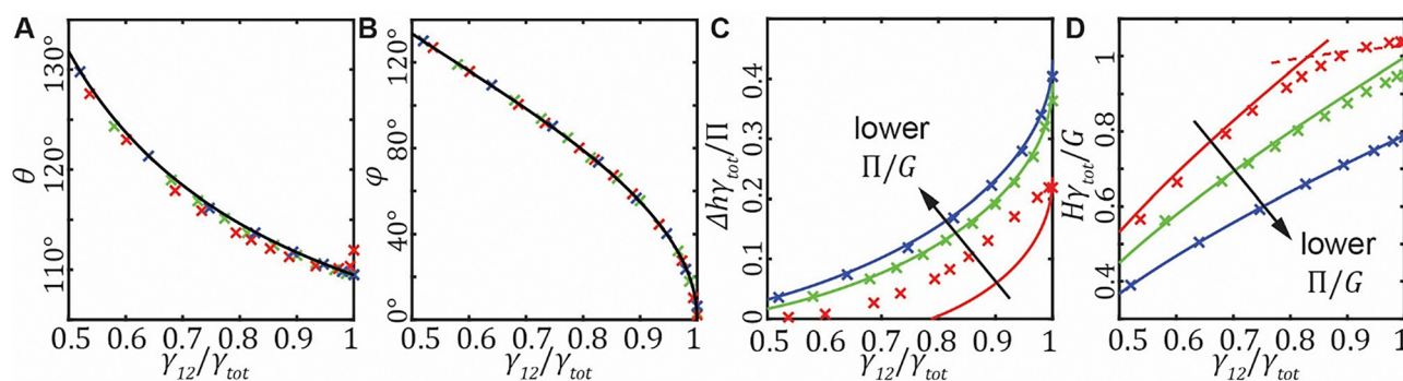
Fig. 4 With \gamma_{S2}/\gamma_{S1} = 2 , how \gamma_{12}/\gamma_{tot} and \Pi/G affect (A) apparent contact angle \theta , (B) tip angle \phi , (C) phase separation size \Delta h , and (D) solid height H . Crosses are simulation results. Solid lines are the analytical solution. The dashed line in (D) is the limiting behavior H = 1.09 \sin \theta \gamma_{tot}/G . Red, green, and blue correspond to \Pi/G = 4, 1, 0.25 .
