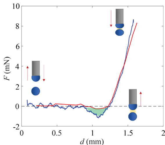
Fig. 5 Force–displacement plot at contact force F_M = 10 mN, relative humidity RH = 80\% , t_c = 1 s and retraction speed v_r = 0.006 mm s −1 . The approach curve is represented by — , and retraction curve by — . The green part represents the area under the F – d plot and hence the total dissipation in the loss of contact. Here, d means the distance by which the upper sphere is lowered respective to the initial position.
