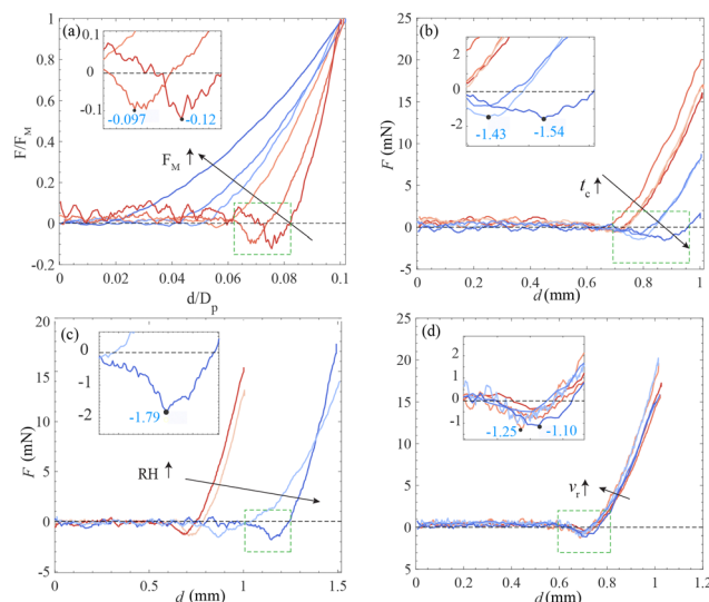
Fig. 6 Force–displacement plots at different (a) contact force F_M = 1, 7, 10, 20, 30, 50, 80 mN, constant RH = 40\% , t_c = 1 s and v_r = 0.006 mm s −1 , (b) contact time t_c = 1, 10, 50, 100, 500, 1000, 2000 s, constant F_M = 10 mN, and v_r = 0.008 mm s −1 , (c) relative humidity RH = 20\%, 40\%, 60\%, 80\% , constant F_M = 10 mN, t_c = 1 s and v_r = 0.006 mm s −1 , and (d) retraction speed v_r = 0.008, 0.006, 0.003, 0.001, 0.05, 0.01 mm s −1 , constant F_M = 10 mN, t_c = 1 s, and RH = 40\% . Insets show close ups of the green dashed-line boxes.
