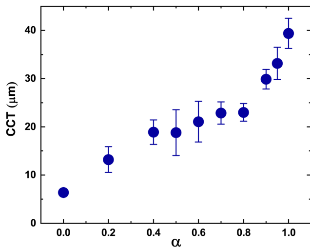
Fig. 4 The measured critical crack-free thickness versus fraction of hard particles ( \alpha ). The CCT was determined using images from microscopy and thickness profiles from profilometry. Films with softer particles crack at lower thickness (low CCT).
