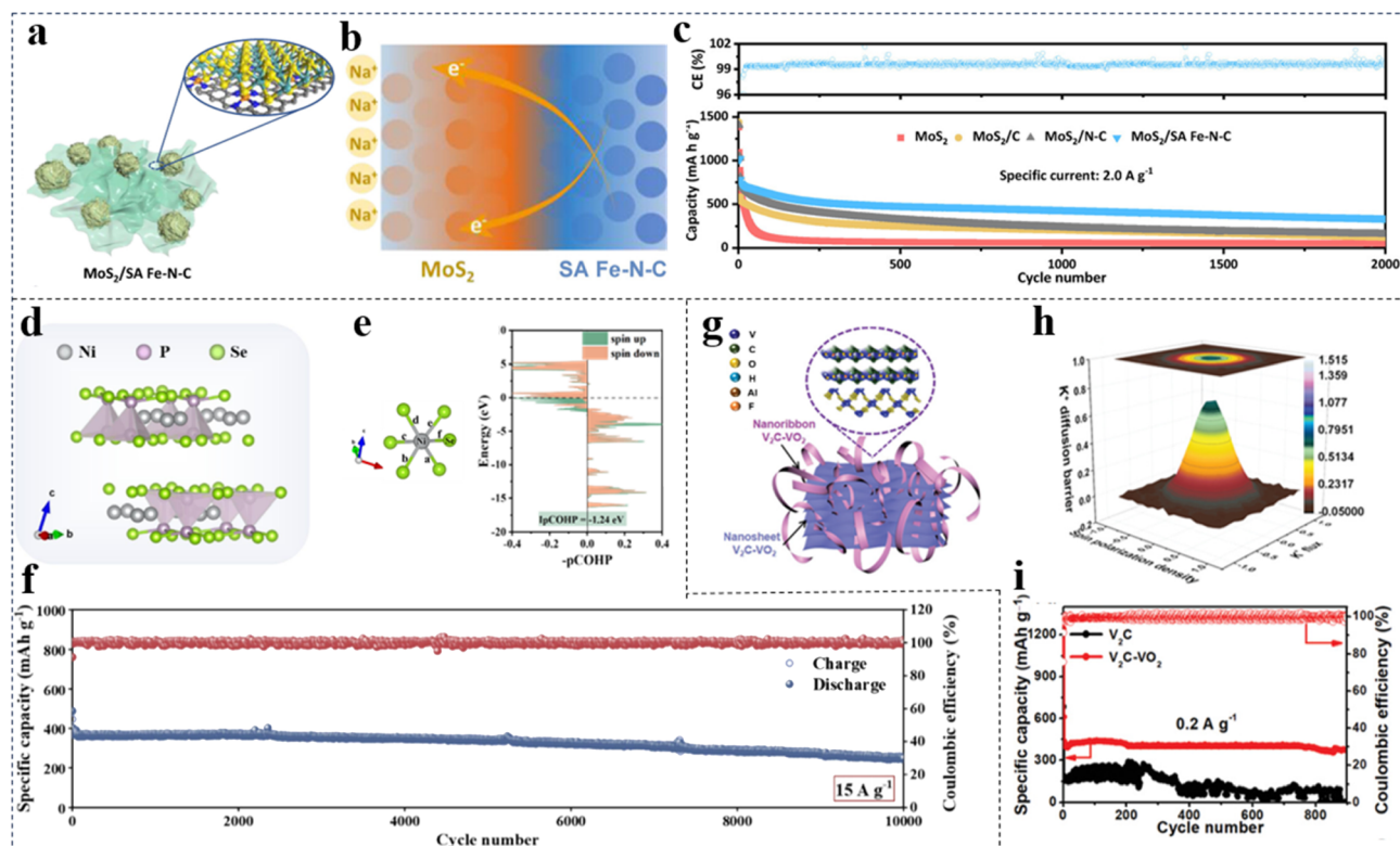
Fig. 16 (a) Schematic illustration of the fabrication of MoS 2 / \text{SA Fe-N-C} . (b) Charge transfer schematic diagram of MoS 2 / \text{SA Fe-N-C} . (c) Cycling performance of MoS 2 / \text{SA Fe-N-C} , MoS 2 / \text{N-C} , MoS 2 / \text{C} , and MoS 2 . Reproduced with permission. 125 Copyright 2023, Wiley-VCH. (d) Schematic diagram of the crystal structure of \text{NiPSe}_3 . (e) Structural model of Ni-Se bonds in \text{NiPSe}_3 . (f) Long-term cycling performance at 15 \text{ A g}^{-1} . Reproduced with permission. 127 Copyright 2025, Elsevier. (g) Schematic illustration of \text{V}_2\text{C-VO}_2 multi-heterostructure. (h) Simulated contour maps of \text{K}^+ ion diffusion barrier versus spin polarization density VH-mode. (i) Cycling stability at 0.2 \text{ A g}^{-1} for \text{V}_2\text{C} and \text{V}_2\text{C-VO}_2 anodes. Cycling stability at 0.2 \text{ A g}^{-1} for \text{V}_2\text{C} and \text{V}_2\text{C-VO}_2 anodes. Reproduced with permission. 130 Copyright 2022, Wiley-VCH.
