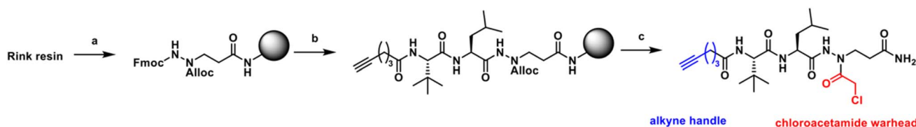
Fig. 13 The synthesis of azapeptide probe 7d . (a) (1) 20% piperidine/DMF; (2) 2-Fmoc-1-allyl-1-(3-(tert-butoxy)-3-oxopropyl)hydrazine-1,2-dicarboxylate, HBTU, DIPEA, DMF, rt, overnight. (b) Repeated cycles: (1) 20% piperidine/DMF, 5 min; (2) Fmoc-Leu-OH; Fmoc-Tle-OH; or hexynoic acid - 3 h, HBTU, DIPEA, DMF, rt. (c) (1) Pd(PPh 3 ) 4 , PhSiH 3 , DCM, 30 min; (2) chloroacetyl chloride, DIPEA, DCM, rt, overnight; (3) TFA/TIPS/water 95/2.5/2.5, 30 min.
