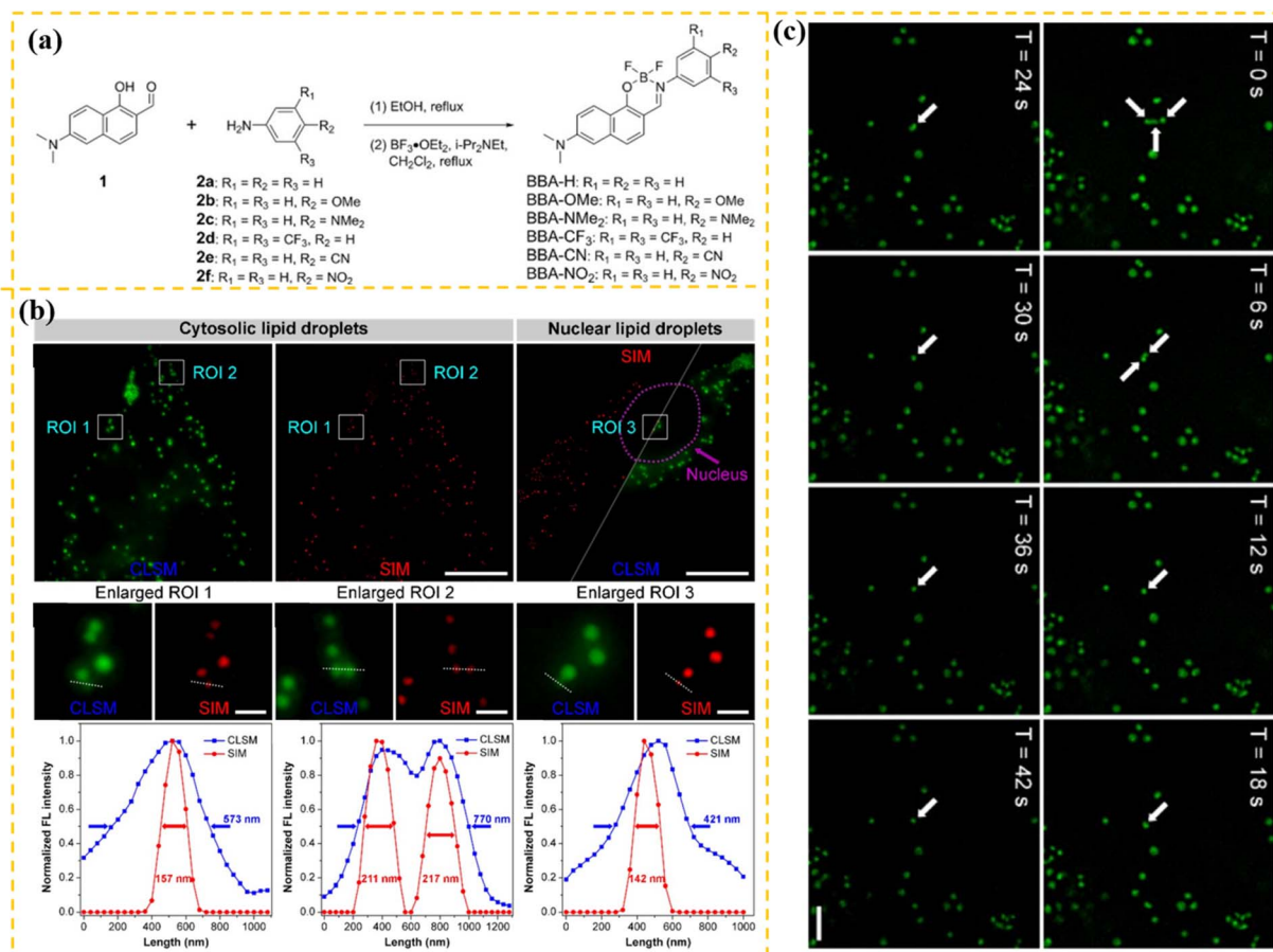
Fig. 30 (a) Synthesis route of probe BBA. (b) Super-resolution fluorescence imaging of probe BBA- \text{CF}_3 in HeLa cells following oleic acid stimulation. (c) Dynamic tracking process of probe BBA- \text{CF}_3 in HeLa cells following oleic acid stimulation. Reprinted with permission from the American Chemical Society, copyright 2022, as cited in ref. 87.
