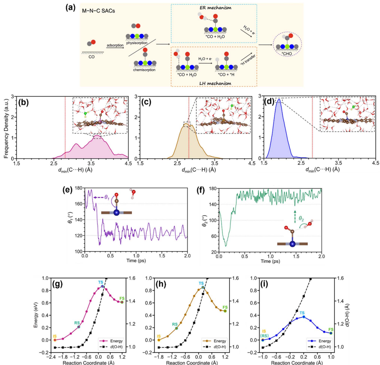
Fig. 10 (a) Schematic diagram of the mechanistic pathways of CO reduction to ^*CHO via the ER and LH mechanisms on M-N-C SACs. 117 (b)–(d) Frequency density distribution of d_{min}(C...H) for (b) [MnPc]^{2-} , (c) [FePc]^{2-} , and (d) [CoPc]^{2-} in explicit water, respectively. The red dashed lines indicate a d_{min}(C...H) of 2.84 Å. Representative snapshots from the trajectory are presented, showing instances in which d_{min}(C...H) aligns with the peak of the frequency density. The H_2O closest to ^*CO is highlighted. (e) and (f) The evolution of the Co–C–O angle ( \theta_1 ) and the C...H–O angle ( \theta_2 ) during the first 2 ps of the molecular dynamics simulation. Snapshots of the Co atom with ^*CO and the closest H_2O are included, corresponding to the simulation time indicated by the arrowheads. (g)–(i) Free energy profile and evolution of average d(O-H) along the reaction coordinate for (g) FePc, (h) MnPc, and (i) CoPc systems. The reaction coordinate is quantified by the collective variable of \xi = d(O-H) - d(C-H) . 119 Reproduced from ref. 117 and 119 with permission from American Chemical Society, copyright 2023, 2024.
