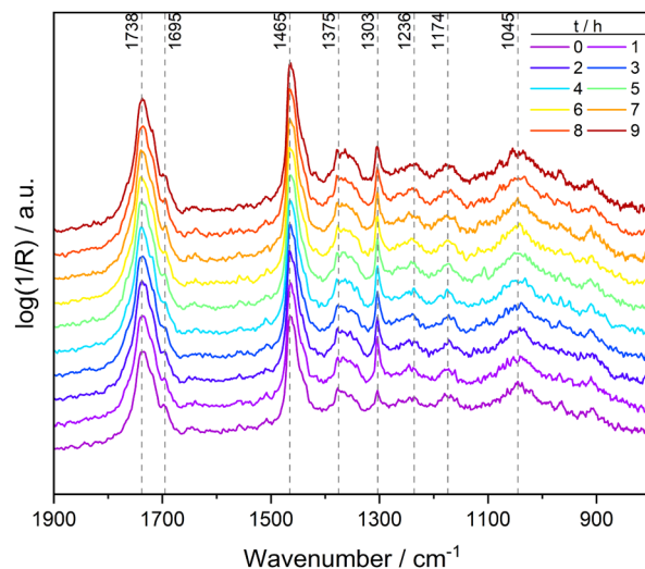
Fig. 2 DRIFT spectra obtained during the induction period at a temperature of 260\text{ }^\circ\text{C} , a \text{H}_2/\text{CO} ratio of 1, 20\text{ cm}^3\text{ min}^{-1} syngas and a pressure of 60 bar.
