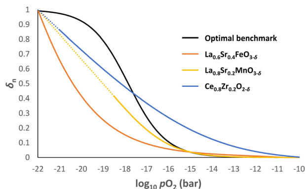
Fig. 8 \delta vs. \log_{10} p_{\text{O}_2} profiles for \text{La}_{0.6}\text{Sr}_{0.4}\text{FeO}_{3-\delta} , \text{La}_{0.8}\text{Sr}_{0.2}\text{MnO}_{3-\delta} and \text{Ce}_{0.8}\text{Zr}_{0.2}\text{O}_{2-\delta} at 1093 K using data from literature. 26,29,32 The optimal \delta - p_{\text{O}_2} relationship is also given as a benchmark. The dotted lines for \text{La}_{0.8}\text{Sr}_{0.2}\text{MnO}_{3-\delta} and \text{Ce}_{0.8}\text{Zr}_{0.2}\text{O}_{2-\delta} indicate extrapolation of the data if no decomposition were to occur.
