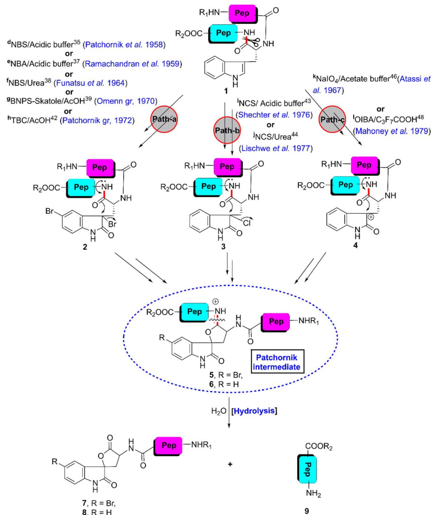
Fig. 2 W-selective scissoring of peptides/proteins through chemical oxidation. [Reaction conditions: ^d NBS, aqueous acetate buffer (pH 4), RT, <1 min, 5–8%; ^e NBA, acidic buffer (pH 4), RT, 15–20 min, 20–40%; ^f NBS, 8 (M) aqueous urea, RT, 200 min, yield not reported; ^g BNPS-skatole/AcOH, RT, 20–30 min, 15%; ^h TBC/AcOH (pH 3), RT, 5–15 min, 50%; ^i NCS/50–80% acetic acid (pH 4–5), RT, 30 min, 35–40%; ^j NCS, 4.68 (M) urea, 27.5% acetic acid, RT, 30 min, 50%; ^k NaIO 4 , acetate buffer (pH 5), 0 °C, followed by acidic hydrolysis at RT, 92–94% at W-7 & 17–22% at W-14 of SWM; ^l OIBA, 80% acetic acid, RT, 30 min, 70–100%].
