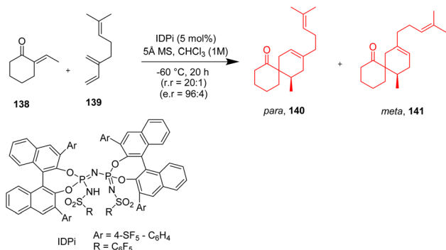
Scheme 18 Enantioselective intermolecular Diels-Alder reaction to form spirocycloclanes ( 140 , 141 ). 50
