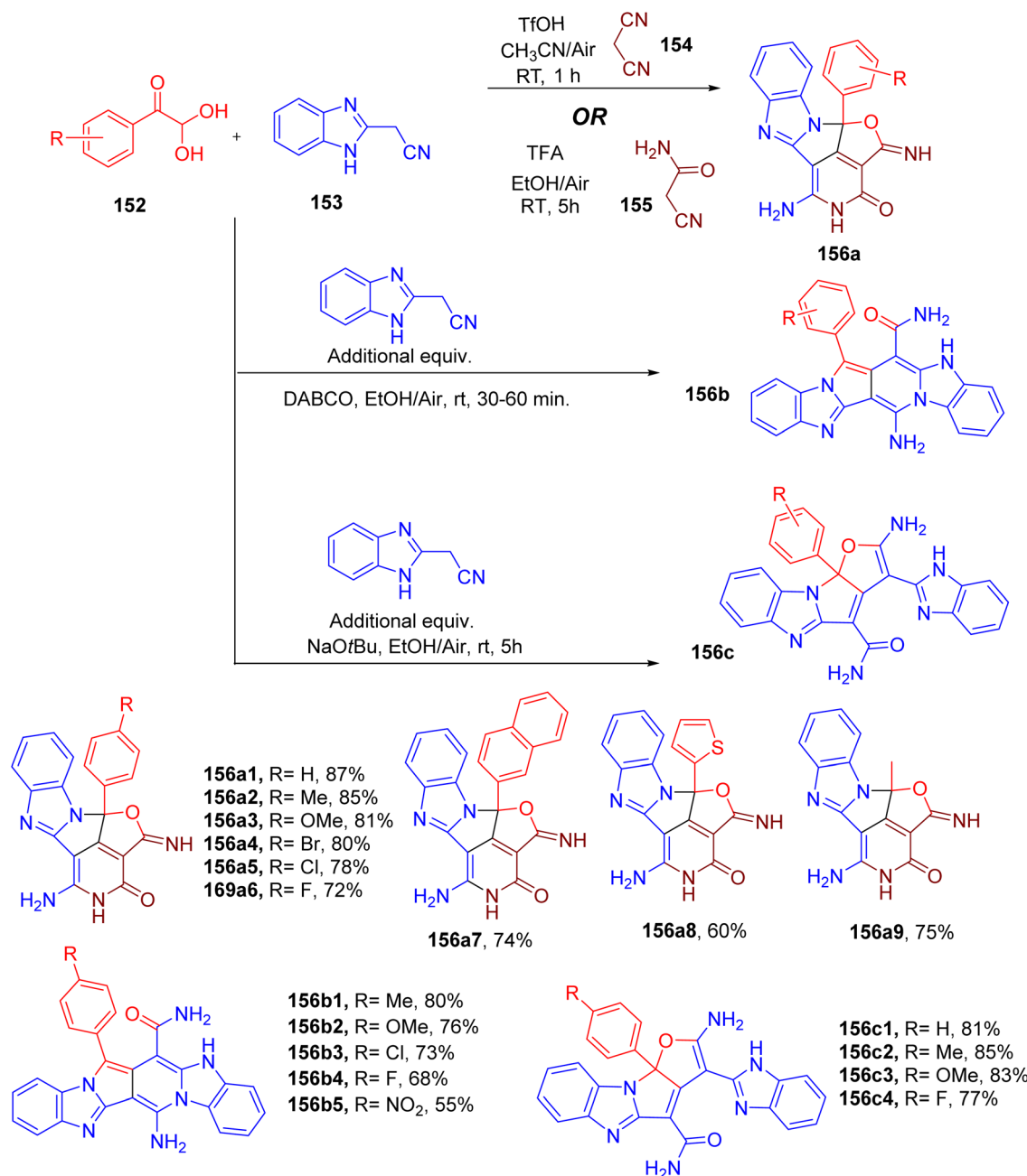
Fig. 39 MCR for the synthesis of aza-cyclopenta(cd)indene ( 156a ), pyrrolo(3,4- d )pyridine-13-carboxamide ( 156b ), and furo-pyrrolo(1,2- a )imidazole-4-carboxamide ( 156c ) scaffolds.
