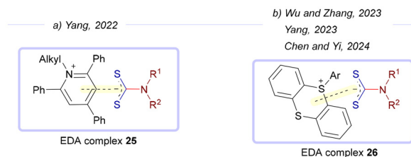
Scheme 4 Dithiocarbamates as electron donors in the reaction between Katritzky salts or thianthrenium salts.
