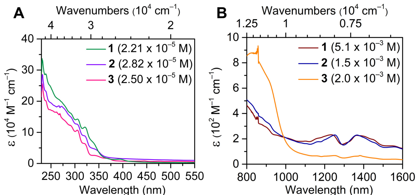
Fig. 6 (A) UV-Vis spectra of [K(DME)_2][U(dbCOT)_2] , 1 (green line), [K(crypt-222)][U(dbCOT)_2] , 2 (purple line), and [K(crypt-222)][U(dbCOT)_2(THF)] , 3 (pink line), in 2-MeTHF solution. (B) NIR spectra of [K(DME)_2][U(dbCOT)_2] , 1 (maroon line), [K(crypt-222)][U(dbCOT)_2] , 2 (blue line), and [K(crypt-222)][U(dbCOT)_2(THF)] , 3 (orange line).
