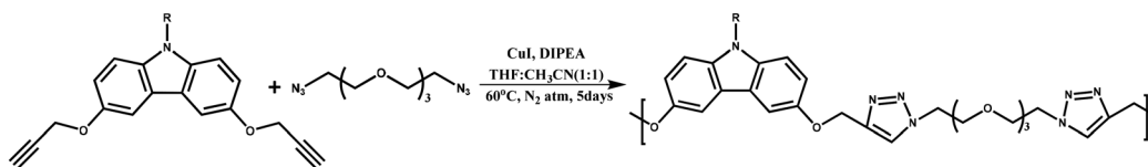
Scheme 2 Synthesis of a donor-bearing polymer by a reaction of 3,6-dipropargyloxy-9-alkyl-carbazole and tetraethylene glycol diazide, using a Cu-catalyzed alkyne-azide click reaction.
