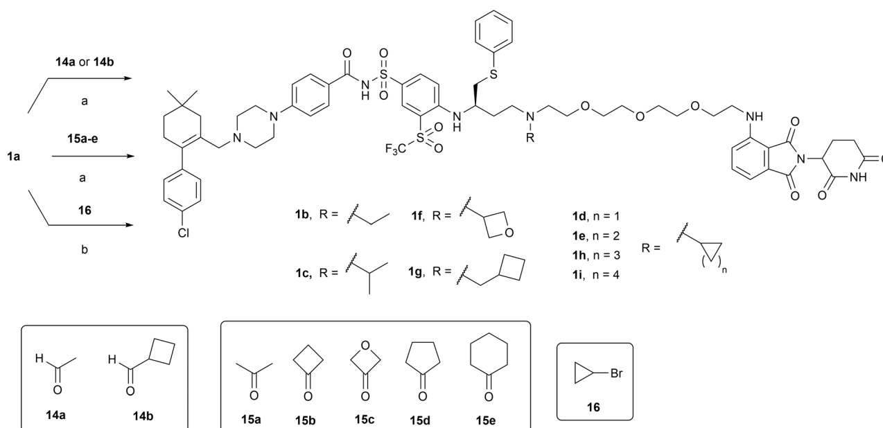
Scheme 2 Reagents and conditions: (a) \text{NaBH}(\text{OAc})_3 , DCE, 50 °C; (b) DIPEA, EtOH, 65 °C.
