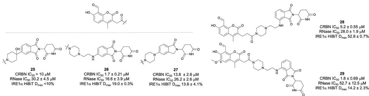
Fig. 4 Biological profiles of IRE1 \alpha PROTACs 25–29. Potency values are shown for CRBN cell-based occupancy (NanoBRET), inhibition of RNase activity and IRE1 \alpha HiBiT D_{\max} (maximum percentage degraded, 24 h treatment, maximum concentration 30 \mu M).
