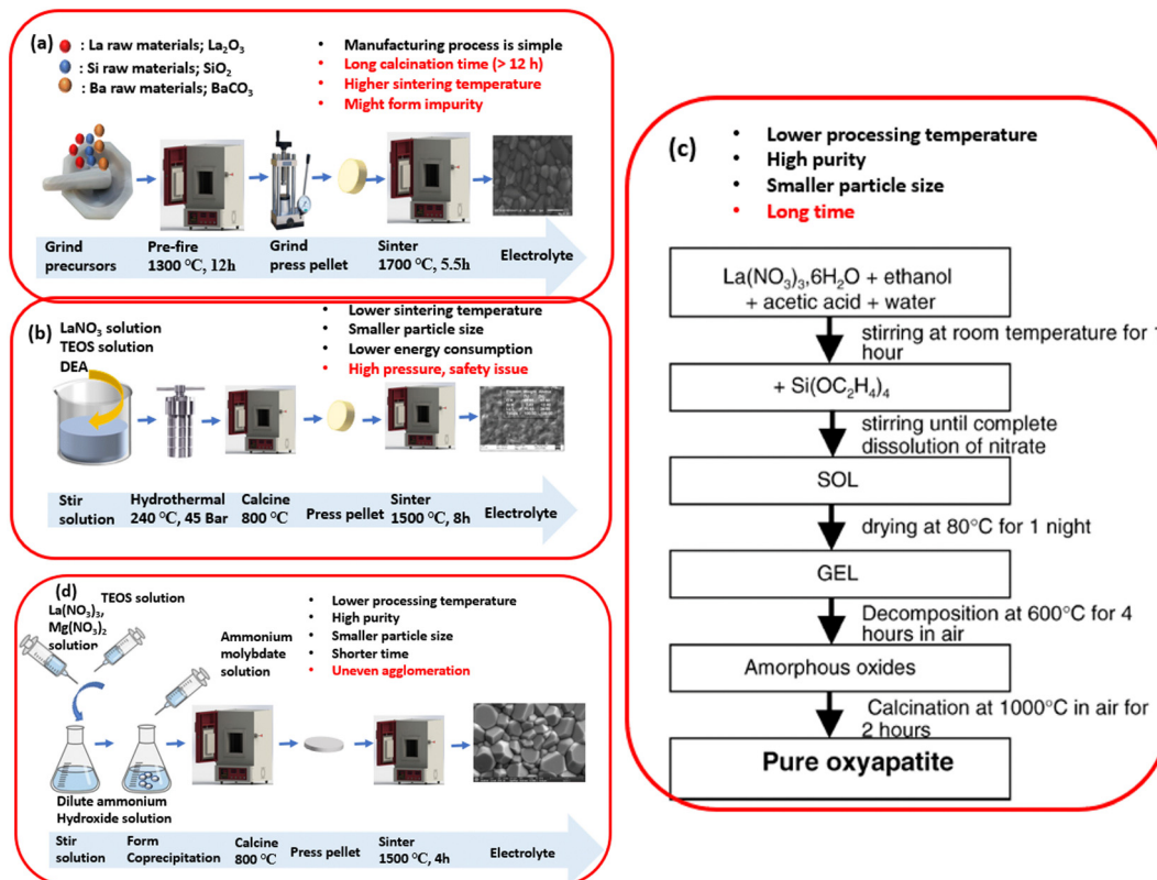
Fig. 12 A schematic of different electrolyte preparation methods: (a) solid-state reaction; (b) hydrothermal synthesis; (c) sol-gel process; (d) co-precipitation method; and the comparison of these methods. 224 Reproduced from ref. 224 with permission from [Elsevier], copyright [2005].
