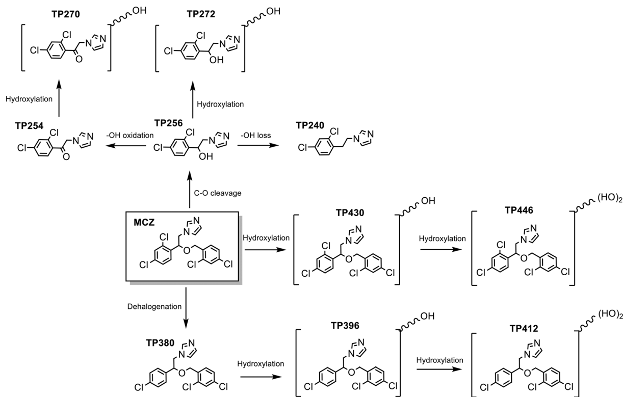
Fig. 6 Miconazole intermediates and degradation pathways during the electro Fenton process of 50 \text{ mg L}^{-1} MCZ at a constant current intensity of 150 \text{ mA} \text{Fe}^{2+} = 0.2 \text{ mM} \text{Na}_2\text{SO}_4 = 50 \text{ mM} .
