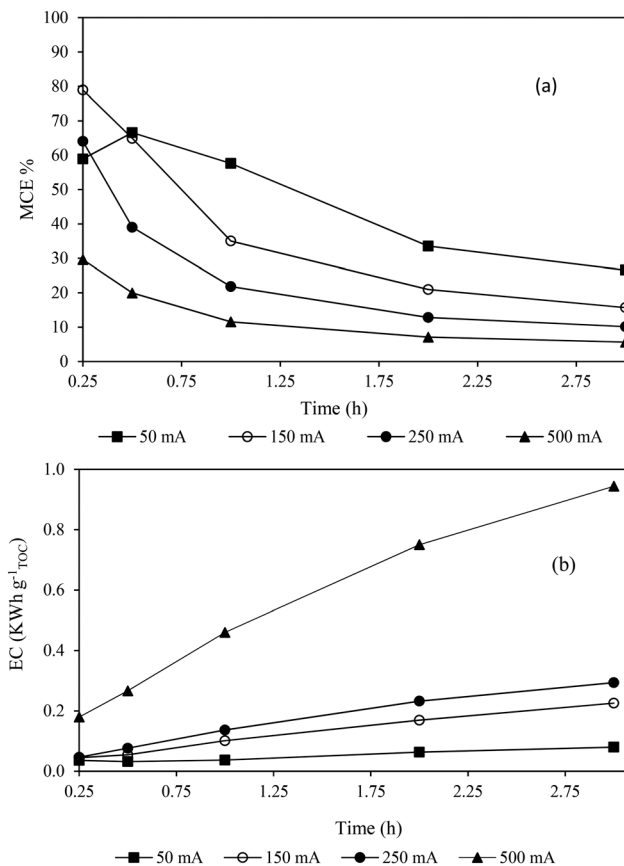
Fig. 3 Mineralization current efficiency (% MCE) (a) and energy consumption ( \text{EC}_{\text{TOC}} ) (b) as a function of electrolysis time of 50 mg L -1 of miconazole corresponding to 25.95 mg L -1 initial TOC by electro-Fenton under operating conditions of [ \text{Na}_2\text{SO}_4 ] = 50 mM, \text{Fe}^{2+} = 0.2 mM and pH = 3.0.
