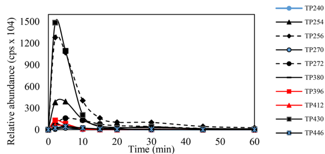
Fig. 7 Time course of formed intermediate compounds during EF treatment of 50 \text{ mg L}^{-1} MCZ at constant current intensity of 150 \text{ mA} \text{Fe}^{2+} = 0.2 \text{ mM} \text{Na}_2\text{SO}_4 = 50 \text{ mM} .
