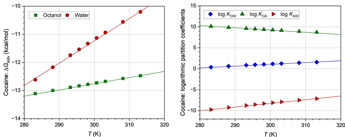
Fig. 6 Left: Temperature dependence of the solvation energies \Delta G_{\text{solv}} for cocaine in water and 1-octanol. Right: Temperature dependence of the cocaine partition coefficients \log K_{\text{OW}} , \log K_{\text{OA}} and \log K_{\text{AW}} . The calculations were performed using COSMO-RS.
