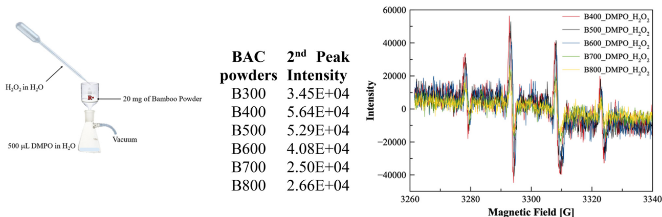
Fig. 10 Schematic illustration for generating stable paramagnetic DMPO - OH species with a sintered glass filter connected to the vacuum system. 20 mg of BAC were weighed into the sintered glass filter, and 500 µL of a diluted H 2 O 2 (2.68 mM) was percolated through it and dropped directly inside a flask containing 0.02 M of DMPO. EPR spectra of DMPO - OH adducts in the final filtered solution (0.02 M of DMPO and 1.34 mM of H 2 O 2 in H 2 O) obtained from different BACs.
