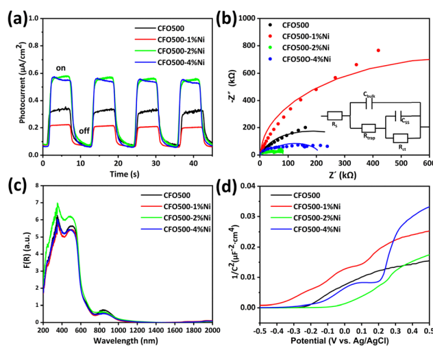
Fig. 3 (a) I - t curves; (b) EIS Nyquist plots under illumination; (c) transformed Kubelka-Munk reflectance spectra of CFO materials; (d) Mott-Schottky plots of CFO500, CFO500-1%Ni, CFO500-2%Ni and CFO500-4%Ni.
