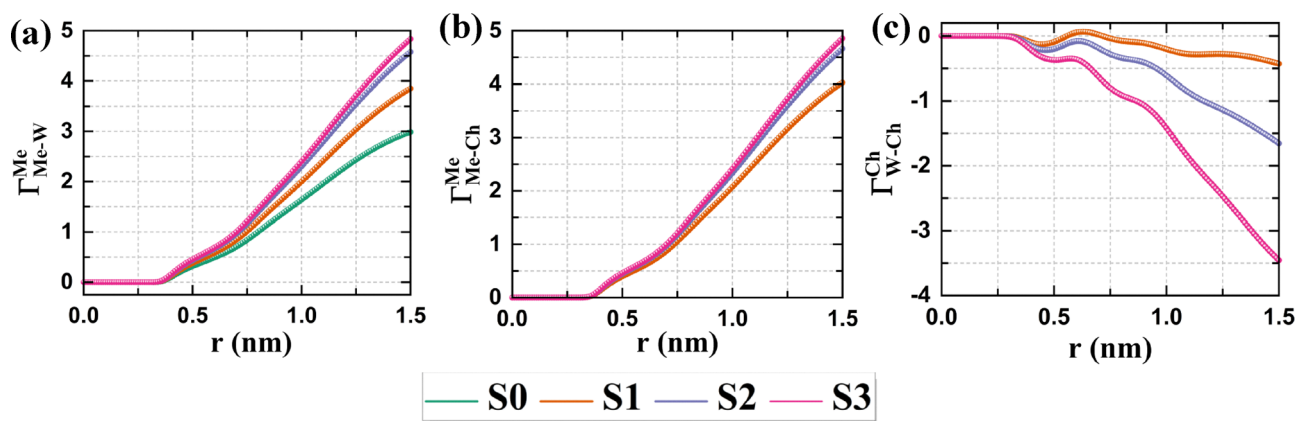
Fig. 7 Preferential interaction parameter for methane considering (a) methane–water, (b) methane–choline and (c) water–choline binary mixtures for all the systems studied.
