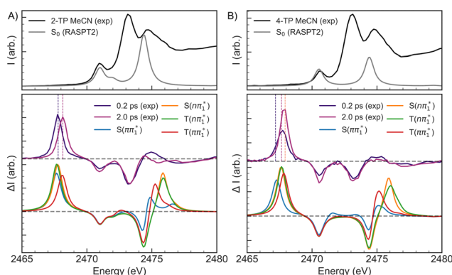
Fig. 5 S K-edge XA spectra of (A) 2-TP impl and (B) 4-TP impl models for the S_1 , S_2 , T_1 and T_2 states. Spectra are calculated at the optimized geometry of the respective valence excited state. The experimental spectra at 0.2 ps, 2 ps are shown for comparison. The dashed lines on the experimental spectra show the peak position obtained from a multi-peak fit to the spectra summarized in Table 2. The energy axis of the theoretical spectra is shifted by 4.45 eV to align the ground state \pi^* resonance with the experiment. Ground state experimental and RASPT2-computed spectra are compared in the top panel (black and gray curves respectively).
