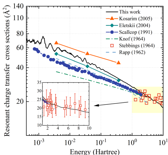
Fig. 4 Comparison of the resonant charge exchange cross sections for the \text{O}(\text{}^3\text{P})\text{--O}^+(\text{}^4\text{S}) interaction as a function of collision energy, where the experimental results are from Stebbings et al. 39 (squares), and the theoretical results are from Kosarim et al. 40 (triangles), Eletsii et al. 9 (rhombuses), Stallcop et al. 18 (cycles), Knof et al. 6 (dot-dashed line), and Rapp et al. 41 (dashed line), respectively.
