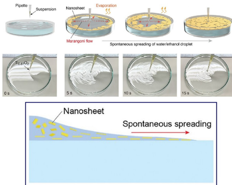
Fig. 4 A method for ultrafast assembly of 2D nanosheet films via spontaneous spreading on a water surface using a water/ethanol suspension containing a cationic surfactant (tetrabutylammonium hydroxide ion) to induce Marangoni-enhanced spontaneous spreading of large uniform 2D films on a water surface within 10 seconds: schematic illustration of spontaneous spreading of 2D nanosheets (top), series of photographs of the spontaneous spreading process (middle), and schematic illustration of the spreading behaviour of a nanosheet suspension (bottom). Reprinted with permission from ref. 44 copyright 2024 Wiley-VCH.
