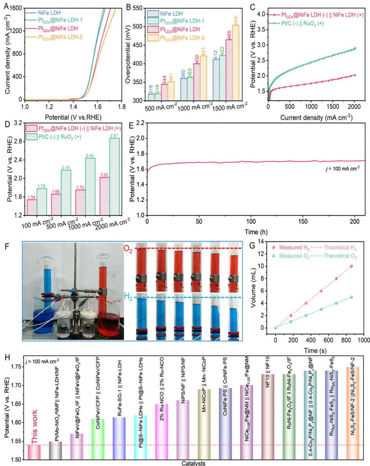
Fig. 11 OWS results; (A) LSV plots; (B) plot depicting comparison of overpotentials at different current densities; (C) potential vs. current density plots \text{Pt}_{\text{ODs}}@/\text{NiFe LDH} (-) || \text{NiFe LDH} (+) and \text{Pt}/\text{C} (-) || \text{RuO}_2 (+) ; (D) plot of potential (cell voltage) vs. current density (E) potential vs. time plot depicting stability in OWS process; (F) snapshots representing the OWS experimental set up and extent of gas collection at different instances; (G) plot depicting measured volume of \text{H}_2 or \text{O}_2 against theoretically produced \text{H}_2 or \text{O}_2 w.r.t. time; (H) potential comparison of \text{Pt}_{\text{ODs}}@/\text{NiFe LDH} (-) || \text{NiFe LDH} (+) over other reported electrocatalysts (reproduced with permission from ref. 61 ©OAE publishing, Inc.; License: CC-BY 4.0).
