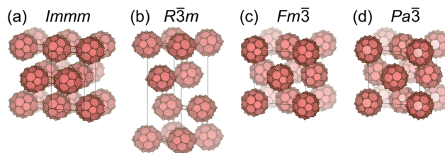
Fig. 14 Crystal structures of solid C_{60} in conventional unit cells with space group (a) Immm , (b) R3m , (c) Fm\bar{3} , and (d) Pa\bar{3} . 220
