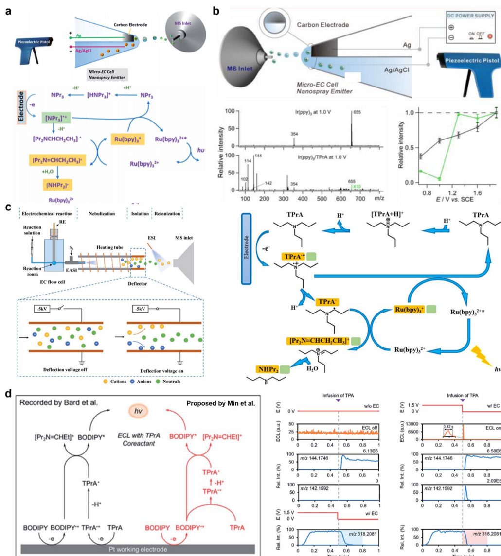
Fig. 14 (a) Schematic illustration of the EC-MS setup containing one micro-carbon electrode and one empty micro-channel, and the “revisited ECL route” of the Ru(bpy)_3^{2+}/TPrA system proposed by Bard. Reprinted with permission from ref. 68. Copyright (2016) The Royal Society of Chemistry. (b) Schematic illustration of the EC-MS setup reported by Shao’s group, the mass spectra of intermediate Ir(ppy)_3^{3+} , and the comparison of the relative intensity of Ir(ppy)_3^{3+} in the presence and absence of TPrA across different potentials. Reprinted with permission from ref. 131. Copyright (2018) American Chemical Society. (c) Schematic diagram of the basic components of the EC-NR-MS setup, and the working principle of the ion deflector, and the ECL pathway of the Ru(bpy)_3^{2+}/TPrA system at a low oxidation potential of 0.8 V. Reprinted with permission from ref. 132. Copyright (2021) The Royal Society of Chemistry. (d) The mechanism for the ECL reaction of the BODIPY/TPrA system proposed by Bard and Min’s group, and the applied potential, ECL-time curve and EICs of characteristic ions obtained by modified RT-Triplex. Reprinted with permission from ref. 77. Copyright (2022) The Royal Society of Chemistry.
