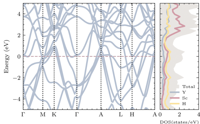
Fig. 3 Electronic band structure of \text{YSc}_2\text{H}_{24} at 310 GPa and projected electronic density of states (PDOS) of each element. The dash line indicates the Fermi level.
