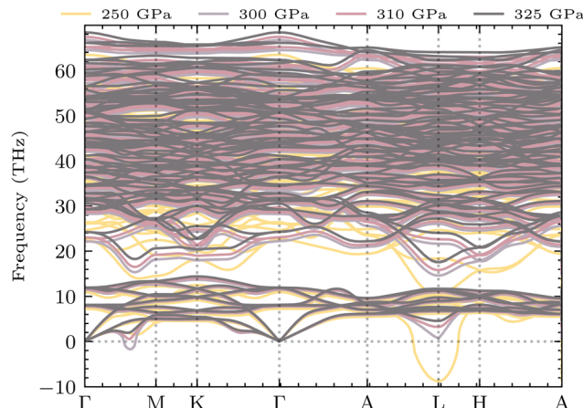
Fig. 4 \text{YSc}_2\text{H}_{24} phonon dispersion at different pressures ranging from 250 to 325 GPa. The region of imaginary frequencies marked by the zero-line frequency reflects the system's dynamic stability. A phonon mode experiences instabilities at 250 GPa, as evidenced by the imaginary mode at the L point of the Brillouin zone. While 300 GPa still shows signs of instability, with imaginary modes present at \Gamma –M or a particularly sensitive imaginary mode at L, at 310 GPa and above, all frequency modes are real, indicating dynamic stability.
