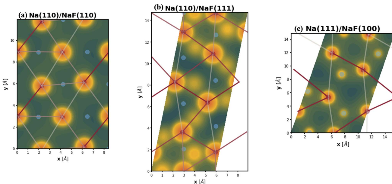
Fig. 4 Contour plots of the logarithm (base 10) of the integrated charge density at the top-most Miller plane of the Na-slabs. Red circles indicate positions of Na atoms of type tag1 and tag2, respectively, while straight lines denote the relative \epsilon_{vv}^{(11)} interactions, with darker, more opaque lines representing stronger interactions. Interfaces represented are (a) Na(110)/NaF(110), (b) Na(110)/NaF(111), and (c) Na(111)/NaF(100). Some of the lines that appear absent are represented through their periodic images.
