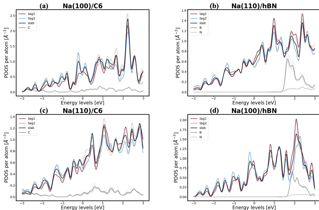
Fig. 7 PDOS for Na/2D systems: (a) Na(100)/C 6 , (b) Na(110)/hBN, (c) Na(110)/C 6 , and (d) Na(100)/hBN. Na atoms on the top and second top-most Miller planes behave exactly like the other Na atoms in the metallic slab, indicating negligible interactions between Na and the 2D materials.
