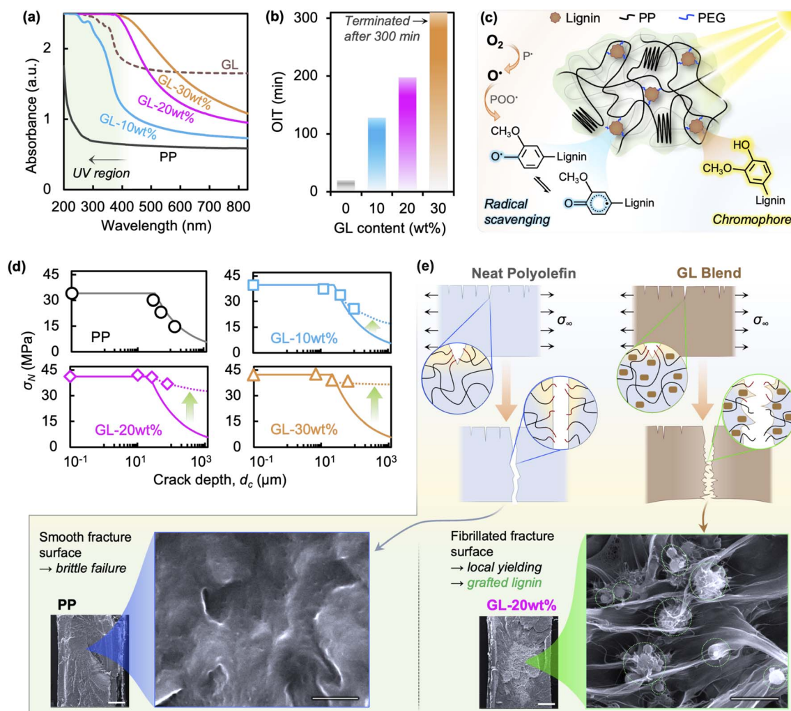
Fig. 5 (a) UV-vis spectra and (b) OIT results for GL/PP blends, and (c) illustration of the simultaneous UV absorber/antioxidant behavior of GL in polyolefin blends. (d) Comparison of experimental (symbols, dotted lines) and analytical (solid lines) values of nominal tensile strength ( \sigma_N ) of neat PP and GL blends as a function of surface crack depth ( d_c ). The deviation from LEFM predictions ( K_{IC} \sim 3.5 \text{ MPa}\sqrt{\text{m}} ) indicates that brittle crack growth does not determine the nominal tensile strength of irradiated GL blends. (e) Illustration of the mechanical reinforcement/toughening effect of GL in polyolefin blends. With sufficient GL loading, well-dispersed lignin particles (circled in green) that are covalently bonded to PP can simultaneously increase stiffness through composite action while blunting crack tips, leading to bulk yielding even when surface cracks are present (see SEM images; scale bars are 2 \mu\text{m} ).
