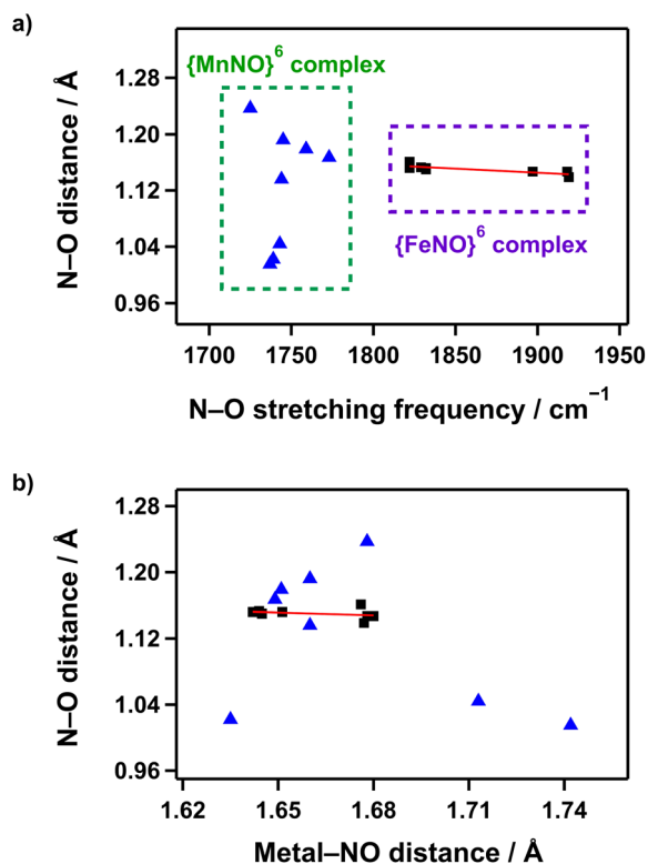
Fig. 6 (a) Plot of the N–O bond distance (Å) against the N–O bond stretching frequency (cm −1 ) for {MnNO} 6 and {FeNO} 6 complexes. (b) Plot of the N–O bond distance (Å) against the M–NO bond length (Å). Triangle (blue) and rectangle (black) represent {MnNO} 6 and {FeNO} 6 complexes, respectively. The solid red line shows a least-squares linear fit of the data.
