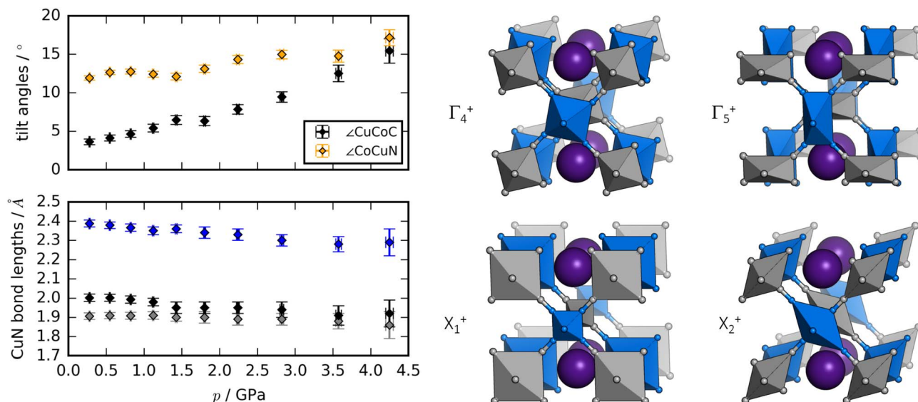
Fig. 3 The left panel shows the pressure evolution of the tilt angles of RbCuCo, with \angle\text{CuCoC} in black and \angle\text{CoCuN} in orange, and the CuN bond lengths of RbCuCo as a function of pressure. The right panel visualises the distortion modes (with exaggerated amplitudes) potentially driving the phase transition in RbCuCo.
