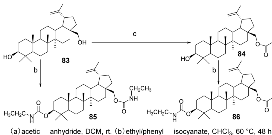
Fig. 25 Synthesis of BA derivatives 85 and 86 .
