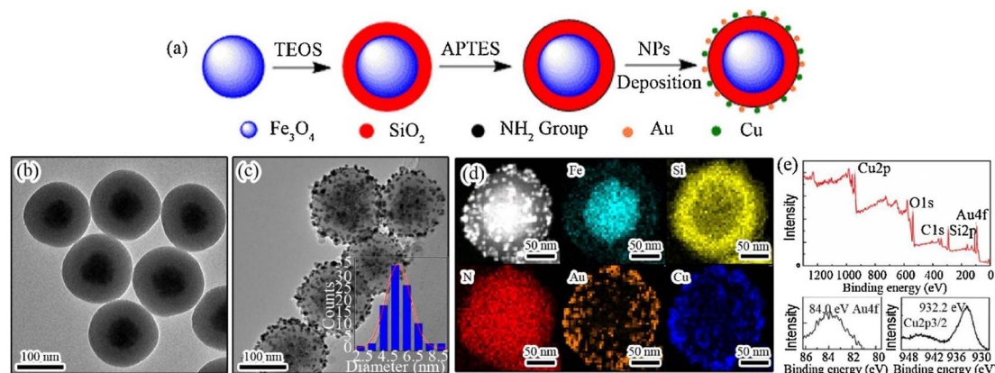
Fig. 6 (a) Stepwise preparation process of \text{Fe}_3\text{O}_4@ \text{SiO}_2 -Au/Cu magnetic nanocomposites. TEM images of (b) \text{Fe}_3\text{O}_4@ \text{SiO}_2 and (c) \text{Fe}_3\text{O}_4@ \text{SiO}_2 -Au/Cu nanoparticles. The inset in (c) depicts the nominal size distribution of Au/Cu NPs over the silica surface, determined by calculating the diameters of around 200 particles in the TEM images. (d) High-angle annular dark-field STEM image of the \text{Fe}_3\text{O}_4@ \text{SiO}_2 -Au/Cu nanocomposite, accompanied by the elemental mapping of Fe, Si, N, Au, and Cu and (e) XPS survey of the \text{Fe}_3\text{O}_4@ \text{SiO}_2 -Au/Cu nanocomposite and high-resolution Au 4f and Cu 2p spectra (adapted with permission from ref. 172, Elsevier, (2018)).
