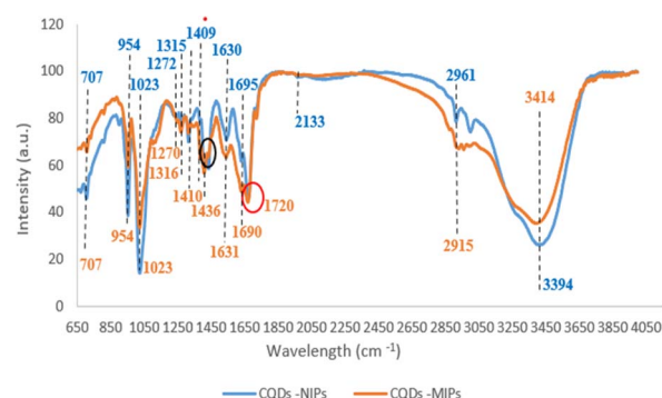
Fig. 2 FT-IR spectra of the CQDs-MIPs and CQDs-MIPs with LSDV.
