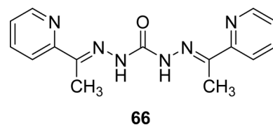
Fig. 38 Structure of Schiff base ligand 66.
