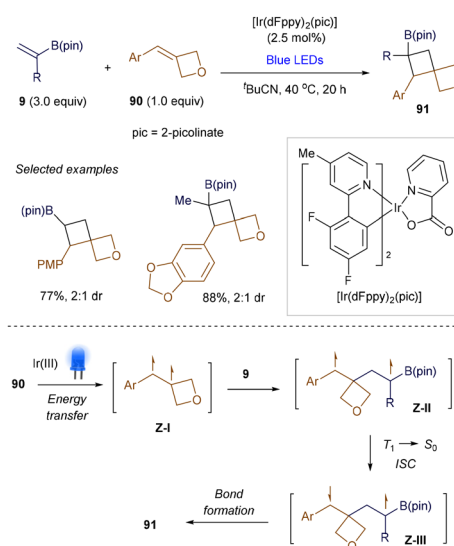
Scheme 34 Catalytic [2 + 2] photocycloaddition.
