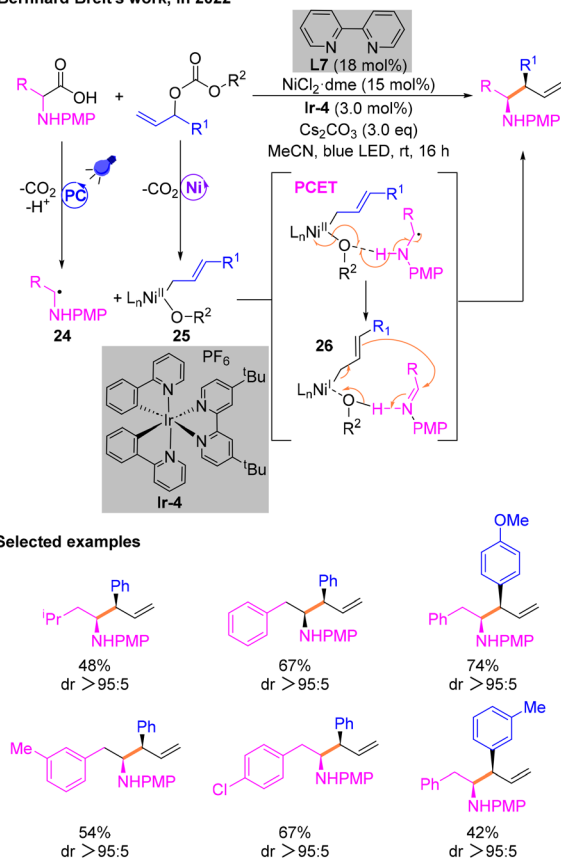
Scheme 10 Synthesis of homoallyl amines by a cross-coupling reaction.
