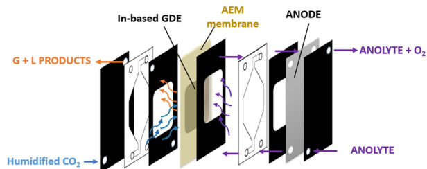
Fig. 2 Schematic view of a continuous flow cell in MEA configuration.
