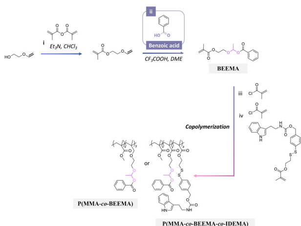
Fig. 25 Scheme of the synthesis of 2-(1-(benzoyloxy)-ethoxyl)ethyl methacrylate (BEEMA) and its copolymerization with either methyl methacrylate or 2-((4-(((2-(1 H -indol-3-yl)ethyl)carbamoyl)oxy)-methyl)phenyl)disulfanyl)ethylmethacrylate (IDEMA) and methyl methacrylate. 179
