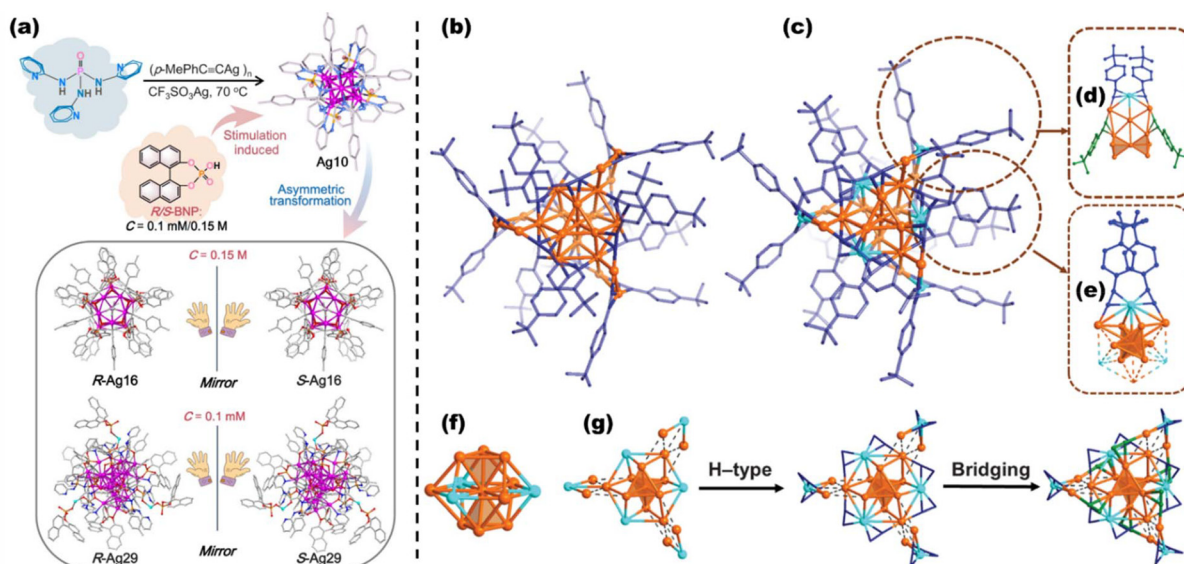
Fig. 7 (a) Varying amounts of R/\text{S-BNP} ligands bring about the asymmetric transformation of achiral \text{Ag}_{10} to chiral R/\text{S-Ag}_{16} and R/\text{S-Ag}_{29} . Reproduced from ref. 155 with permission from the American Chemical Society, copyright (2024). Topological structures of \text{Au}_{22} (b) and \text{Au}_{16}\text{Cu}_6 (c) nanoclusters, H atoms are omitted for clarity. Coordination modes of Cu atoms in the \text{Au}_2\text{Cu} motifs (d) and \text{Au}_6\text{Cu}_6 motifs of \text{Au}_{16}\text{Cu}_6 . (f) \text{Au}_{10}\text{Cu}_3 kernel of \text{Au}_{16}\text{Cu}_6 . (g) Structural evolution of \text{Au}_{16}\text{Cu}_6 , tert -butyl phenyl groups are omitted for clarity. Note: Au = orange; Cu = light blue; C = blue/deep blue or green. Reproduced from ref. 164 with permission from the American Association for the Advancement of Science, copyright (2024).
