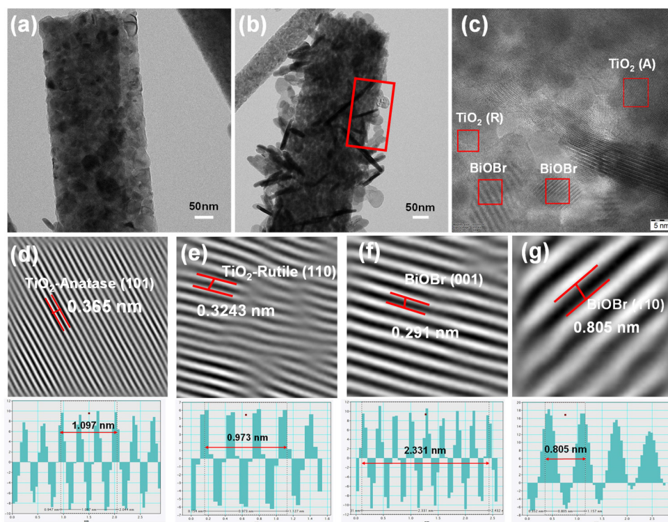
Fig. 5 (a and b) TEM images of TNF and BTNF 1.5 and (c) HRTEM image of BTNF 1.5 . (d–g) Inverse Fourier-filtered images of TiO 2 -anatase, rutile, and BiOBr- (001) and (110) planes with their corresponding line profiles.
