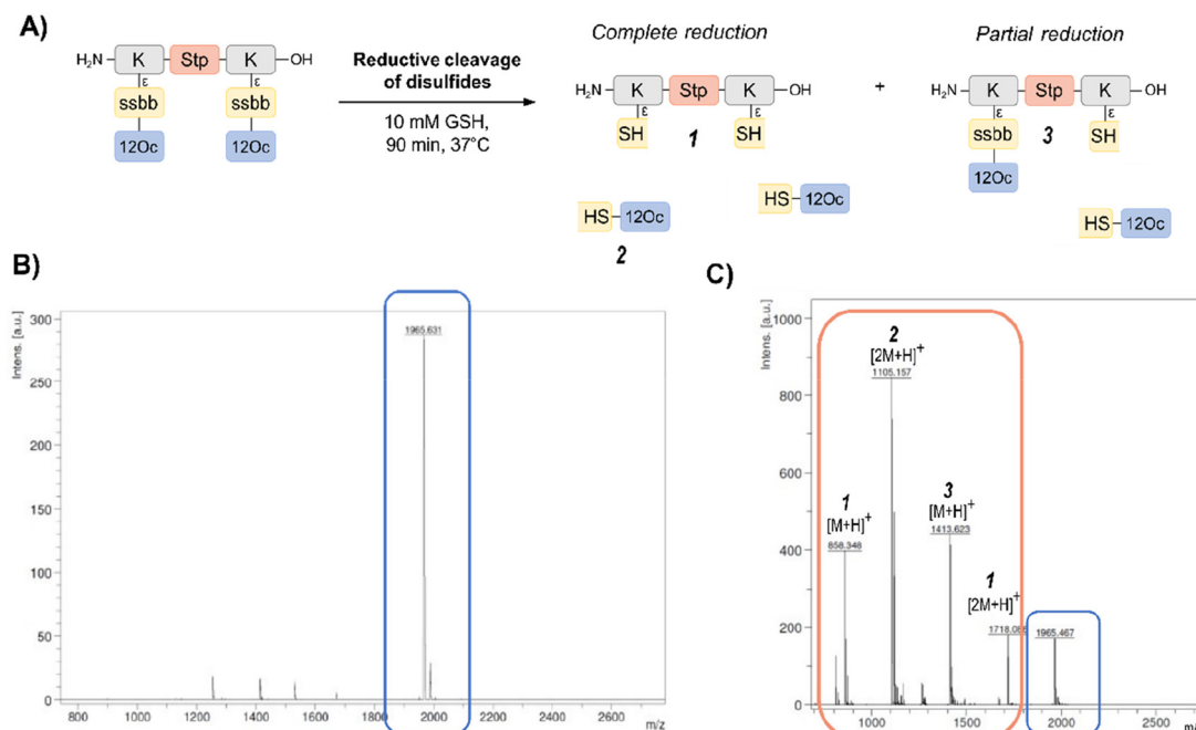
Fig. 1 MALDI analysis before and after incubation with glutathione (GSH). (A) Scheme of disulfide-containing LAF-oligomer 1821 with 12Oc-U1-1:2 topology before and after GSH-induced reduction of disulfides with possible cleavage products upon complete or partial reduction. Representative MALDI mass spectra of disulfide-LAF-oligomer 1821 before (B) and after (C) treatment with 10 mM GSH for 90 min at 37 °C. The mass spectrum after GSH-treatment contains additional peaks (1, 2 and 3) assigned to cleavage products upon disulfide reduction.
