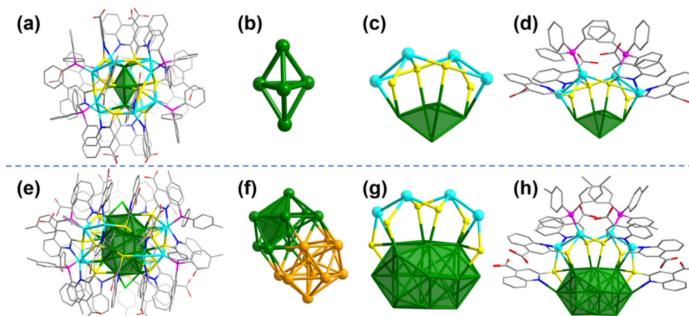
Fig. 2 (a) The overall structure of Ag 17 . (b) The Ag 5 kernel of Ag 17 . (c) The Ag 4 S 4 motif of Ag 17 . (d) The Ag 17 peripheral Ag 4 L 4 (PPh 3 ) 2 unit. (e) The overall structure of Ag 32 . (f) The Ag 20 kernel of Ag 32 (the polyhedron highlighted is an Ag 5 unit). (g) The Ag 4 S 6 motif of Ag 32 . (h) The Ag 32 peripheral Ag 4 L 6 (P(Ph- i -CH 3 ) 3 ) 2 unit. Atom colors: Ag, dark green, turquoise and orange; P, purple; N, blue; S, yellow; Cl, light green; C, gray; O, red. All hydrogen atoms are omitted for clarity.
