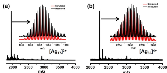
Fig. 1 (a) Positive-ion mode ESI-MS of Ag 17 in CH 3 OH. (Inset) Measured (black line) and simulated (red line) isotopic distribution patterns of the molecular ion peak. (b) Positive-ion mode ESI-MS of Ag 32 in CH 3 OH. (Inset) Measured (black line) and simulated (red line) isotopic distribution patterns of the molecular ion peak.
