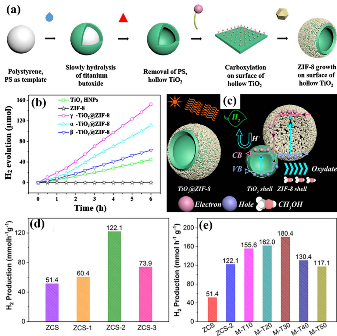
Fig. 18 (a) Diagram showing the incorporation of double-shell \text{TiO}_2 /ZIF-8 hollow nanoparticles. (b) The photocatalytic ability for generating the HER of \text{TiO}_2 HNPs, ZIF-8, and \alpha -/ \beta -/ \gamma - \text{TiO}_2 /ZIF-8. (c) The operation of the HER over \text{TiO}_2 /ZIF-8. Adapted from ref. 389. Copyright © 2019, Elsevier, (d) HER of ZCS composites. (e) ZCS-2, M-TiO 2 , and varied proportions of ZCS-2/M-TiO 2 mixtures. Adapted from ref. 390. Copyright © 2021, Elsevier.
