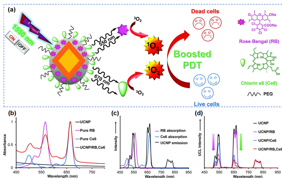
Fig. 8 (a) Schematic diagram of the formation of \text{UCNP}@SiO_2/\text{RB}/\text{Ce6} . (b) The absorbance of UCNPs, RB, Ce6, \text{UCNP}/\text{RB}/\text{Ce6} . (c) The absorption and emission spectra of RB, Ce6 and UCNPs respectively. (d) The UCL spectra of UCNPs, \text{UCNP}/\text{RB} , \text{UCNP}/\text{Ce6} and \text{UCNP}/\text{RB}/\text{Ce6} under irradiation at 1550 nm. Reproduced with permission from ref. 58. Copyright 2014, The Royal Society of Chemistry.
