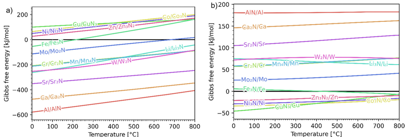
Fig. 2 Ellingham diagrams of the reactions of cycle II for the systems based on Ca, Cr, Mn, Fe, Co, Ni, Cu, Zn, Sr, Mo, W, Li, and Al: (a) standard \Delta G_{\text{rxn}}^{\circ} per mol N 2 as a function of temperature in the range of 0–800 °C for the nitridation reactions according to eqn (2a), and; (b) standard \Delta G_{\text{rxn}}^{\circ} per mol H 2 as a function of temperature in the range of 0–800 °C for the hydrogenation reactions according to eqn (2b). Indicated are the corresponding metal/metal nitride systems.
