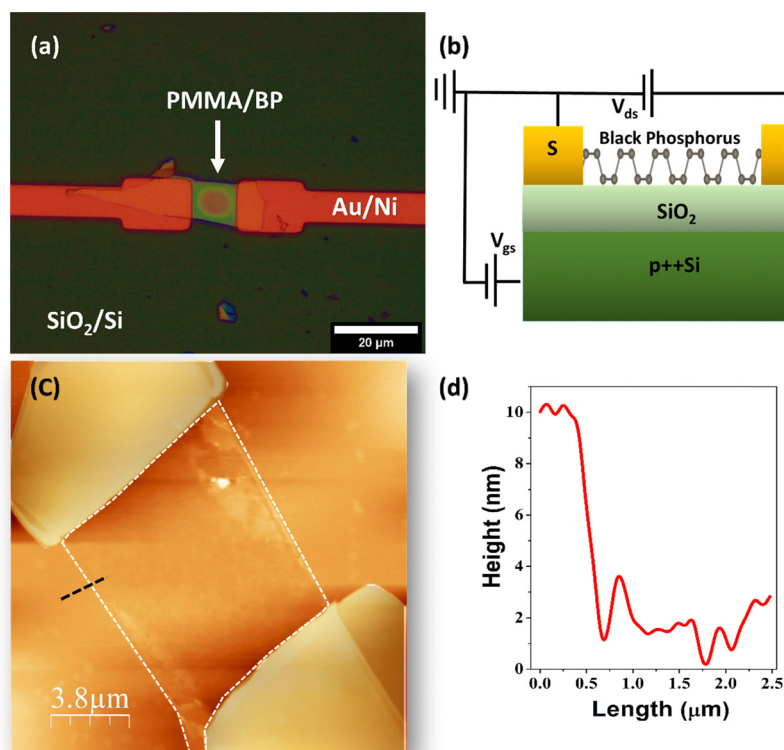
Fig. 1 (a) Optical image of the BP FET device. (b) Schematic diagram of the BP FET device. (c) AFM image of the BP FET device. (d) Height profile along the black line over the BP channel.
